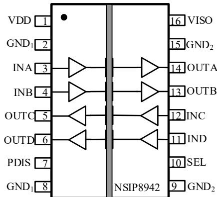
Figure 1.3 NSIP8942 Package
